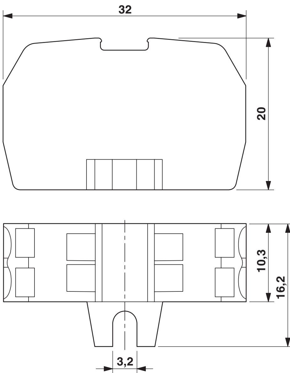
Dimensional drawing
