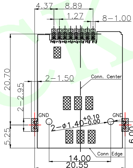
RECOMMENDED PCB LAYOUT(TOP VIEW) GENERAL TOLERANCES:±0.05
