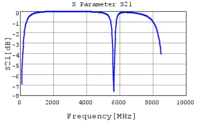
GQM2195G2H8R0DB12 S21 DCOV, 25degC
