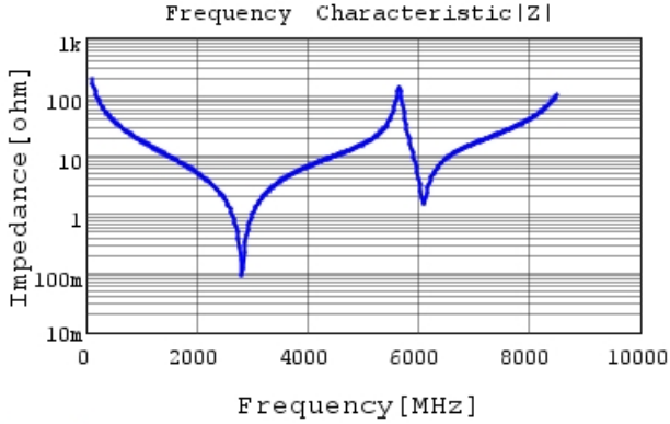
GQM2195G2H8R0DB12 |Z| DCOV, 25degC
