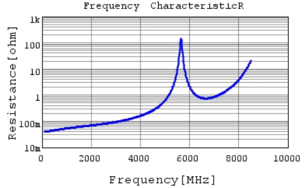
GQM2195G2H8R0DB12 R DCOV, 25degC
