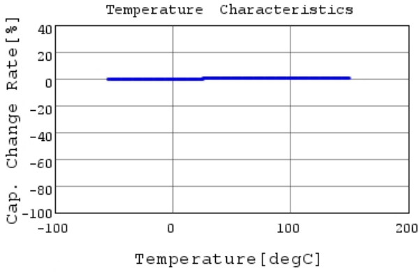
GQM2195G2H8R0DB12 C-Temp. capchange, DCOV, 1
