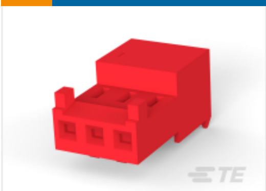
TE Part #3-643815-6 Nylon Tin Plated Receptacle: 2.54 mm, with Mating Alignment, MTA 100
