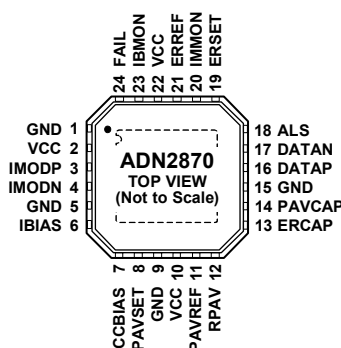
Figure 5. Pin Configuration
