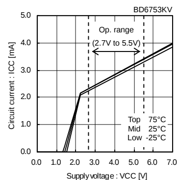
Fig.6 Circuit current
