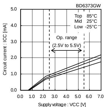
Fig.4 Circuit current
