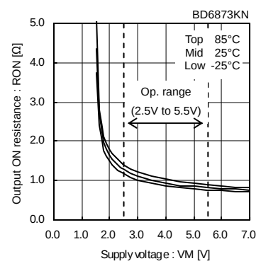
Fig.9 Output ON-Resistance (Linear Constant-Current Drive)
