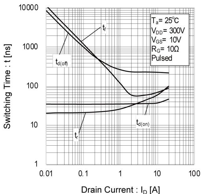
Fig.17 Switching Characteristics
