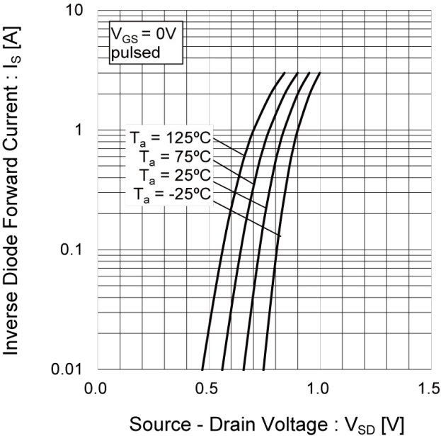
Fig.18 Souce Current vs. Source-Drain Voltage
