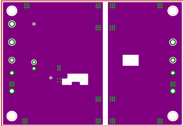
Figure 9. Middle Layer2 Layout (Top View)
