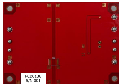
Figure 2. BD7F200HFN-EVK-002 Evaluation Board
