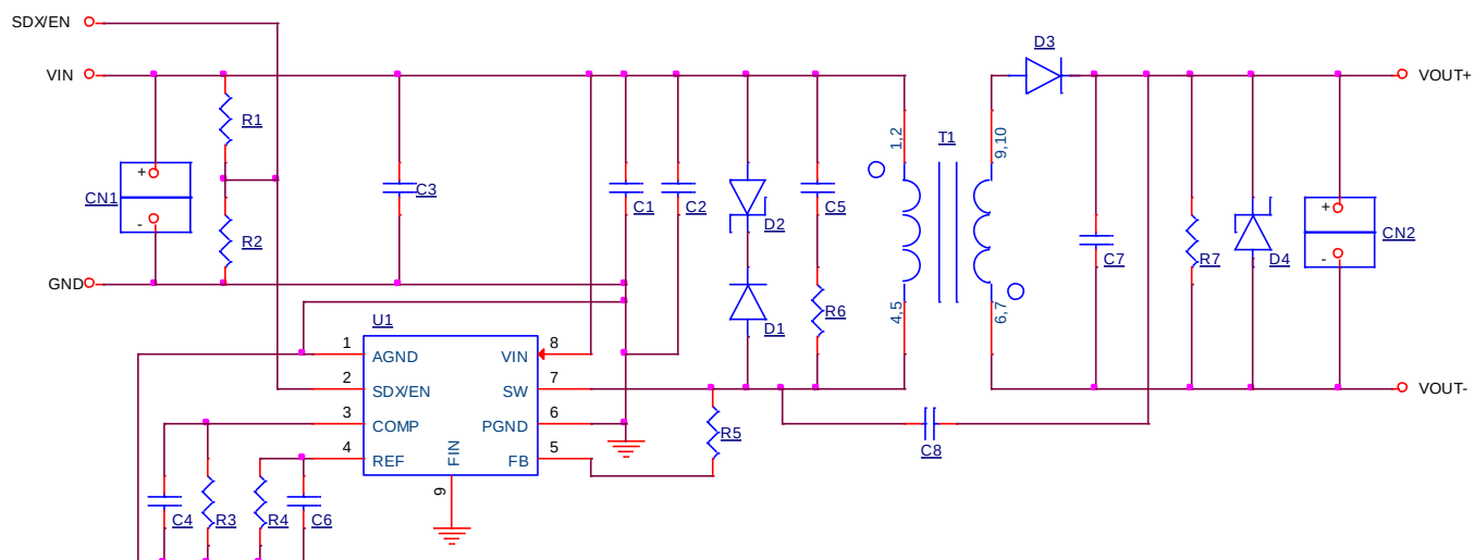
Figure 4. BD7F200HFN-EVK-002 Circuit Diagram
