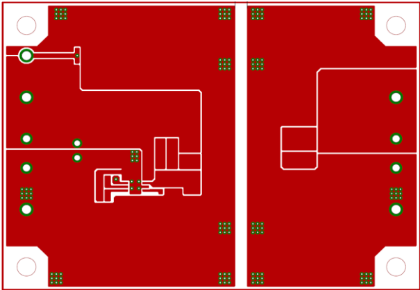
Figure 7. Top Side Layout (Top View)
