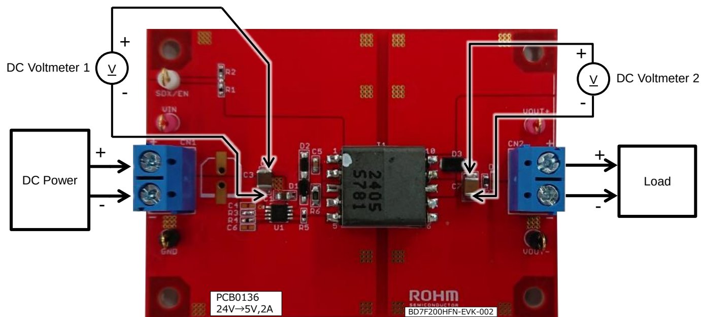
Figure 3. Connection Diagram
