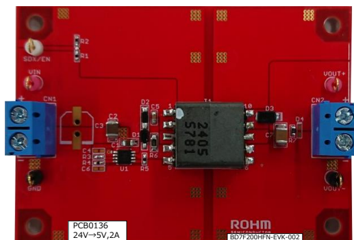
Figure 1. BD7F200HFN-EVK-002 Evaluation Board
