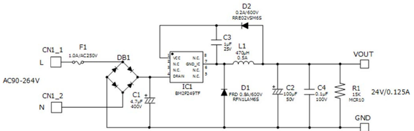
Figure 3. BM2P249TF-EVK-001 Schematics
