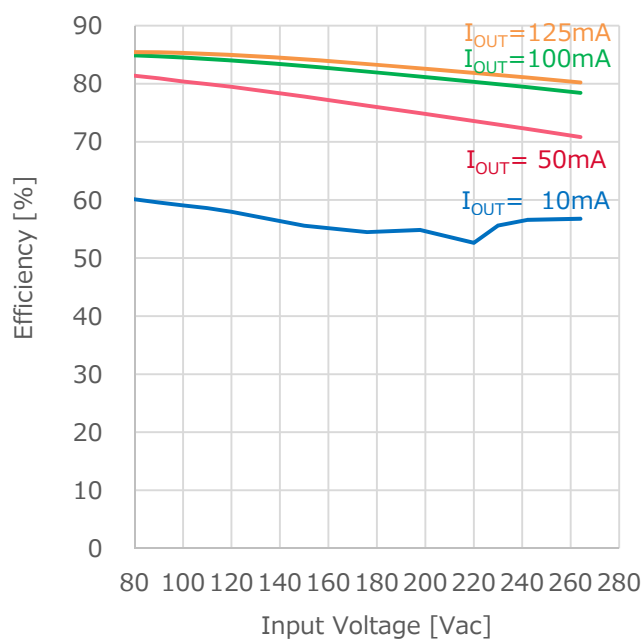
Figure 11. LINE Regulation ( I_{IN} vs. Efficiency)
