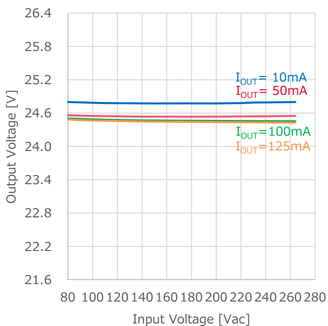
Figure 10. LINE Regulation ( I_{IN} vs. V_{OUT} )
