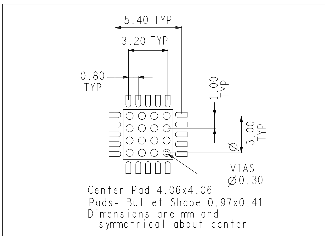
Figure 5-1. Recommended Surface Mount Land Pattern for 20-Pin QFN
