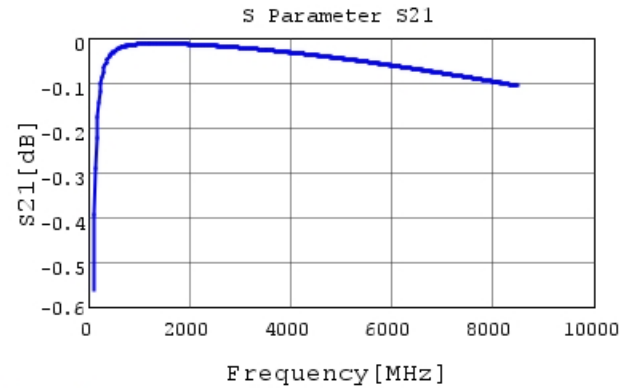
GRM0115C1E430JE01 S21 DCOV, 25degC
