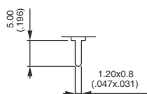
Straight PC
