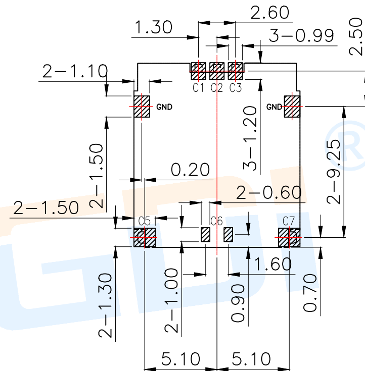
RECOMMENDED PCB LAYOUT GENERAL TOLERANCE \pm 0.05
