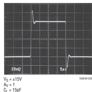
Small-Signal Response
