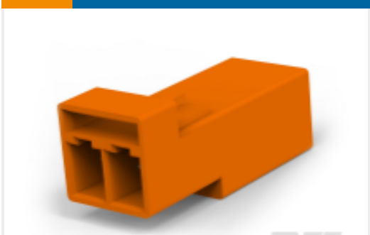
TE Part #1-2834049-4 Modular Latched Receptacles, LIGHT-N-LOK
