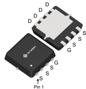
DFN3X3-8L (VSONP-8(3.3x3.3))
