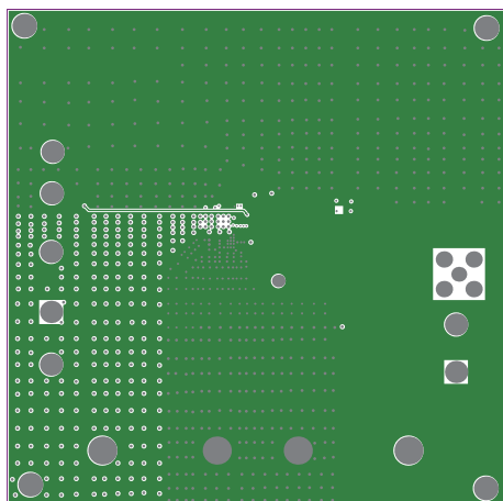
Figure 3: Inner Layer 1
