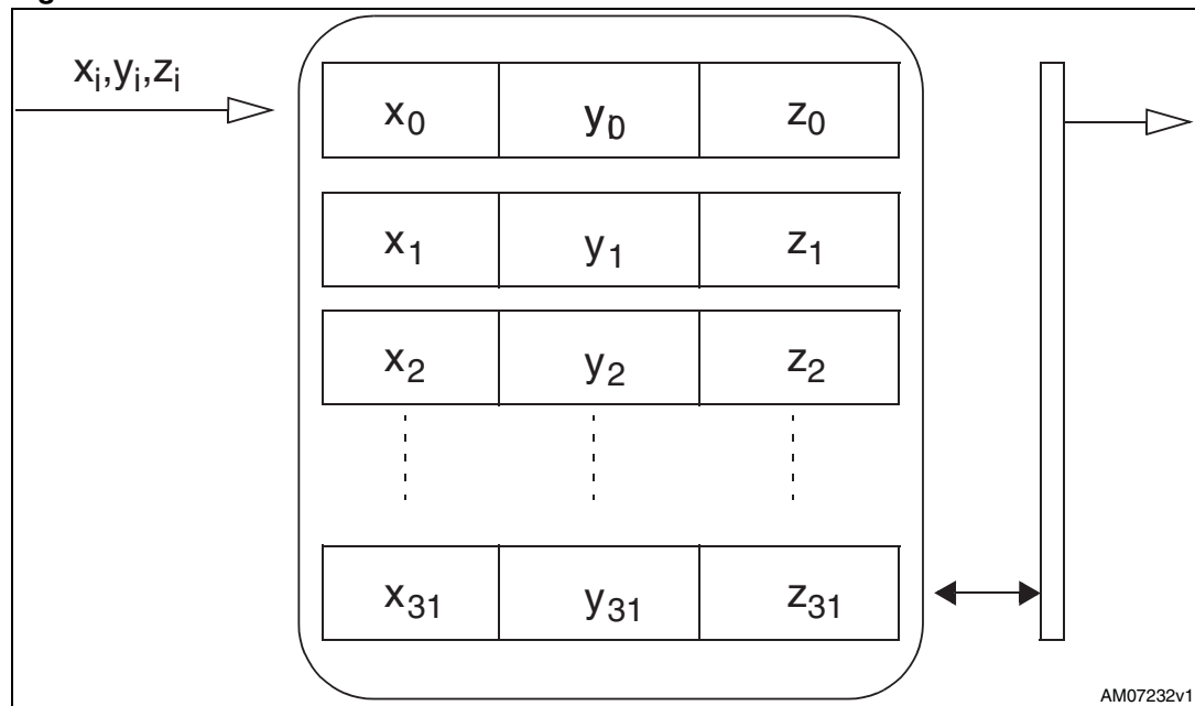
Figure 8. FIFO mode
