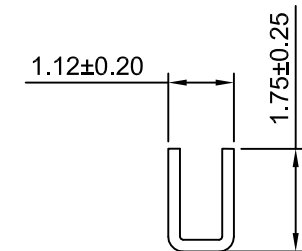
SEC:C-C
