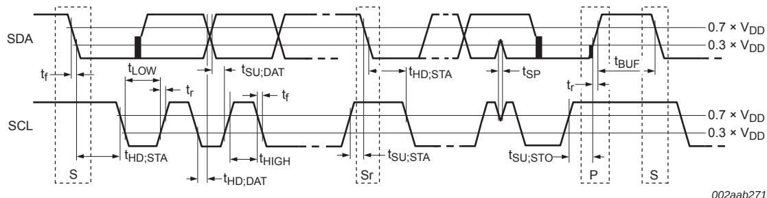
Fig 20. Timing diagram
