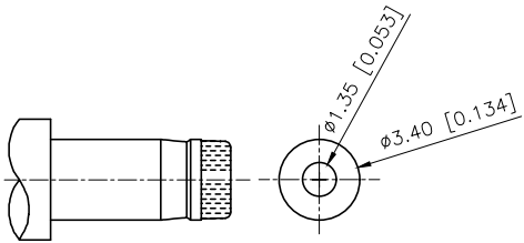
MATING PLUG Jack Insertion Depth: 9.15 mm
