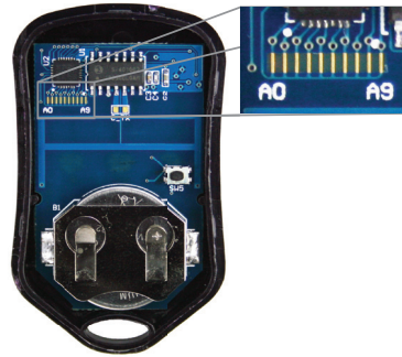
Figure 5: Address Traces
