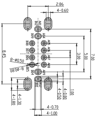
RECOMMENDED P.C.B. LAYOUT (俯视图) TOLERANCE UNSPECIFIED ±0.05mm
