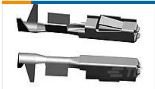
TE Part #929008-2 MQS1MM BU-KONT 90GR
