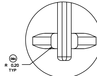
VIEW L
