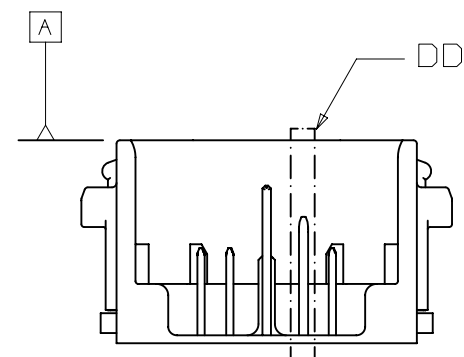
SECTION CC-CC
