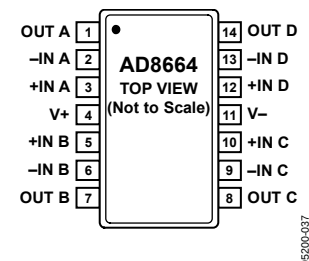
Figure 6. AD8664, 14-Lead TSSOP (RU-14)
