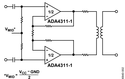
Figure 2. Typical PLC Driver Application
