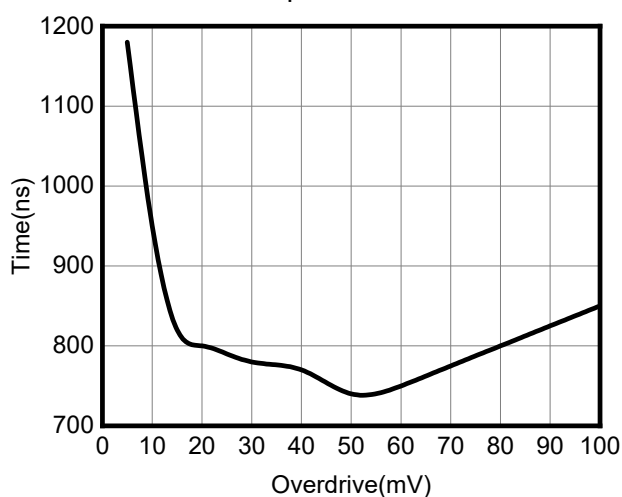
Figure 5. Response Time vs Input Overdrives Positive Transition ( V_{CC}=5\text{V} )
