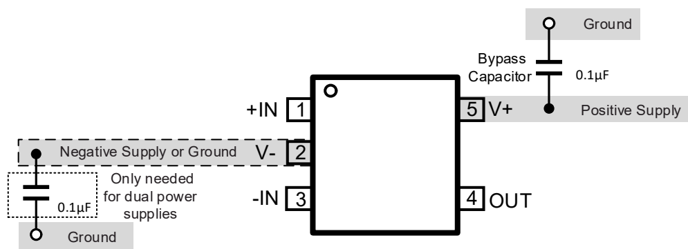
Figure 11. LMV331 Layout Example
