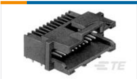
TE Part #5-104069-7 60 sys 50 HDR DRRA SHRD SN
