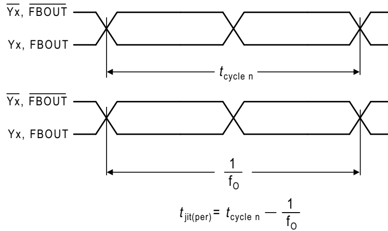
Figure 6. Period Jitter
