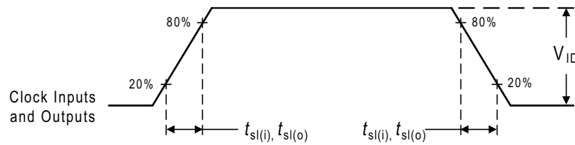
Figure 8. Input and Output Slew Rates
