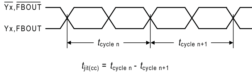
Figure 3. Cycle-to-Cycle Jitter
