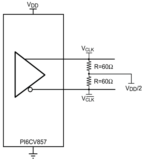
Figure 1. IBIS Model Output Load
