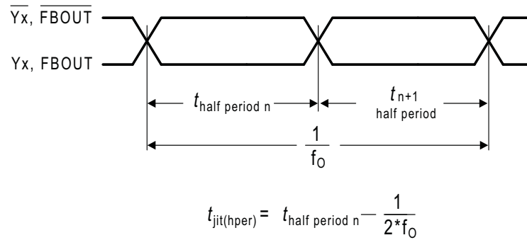
Figure 7. Half-Period Jitter
