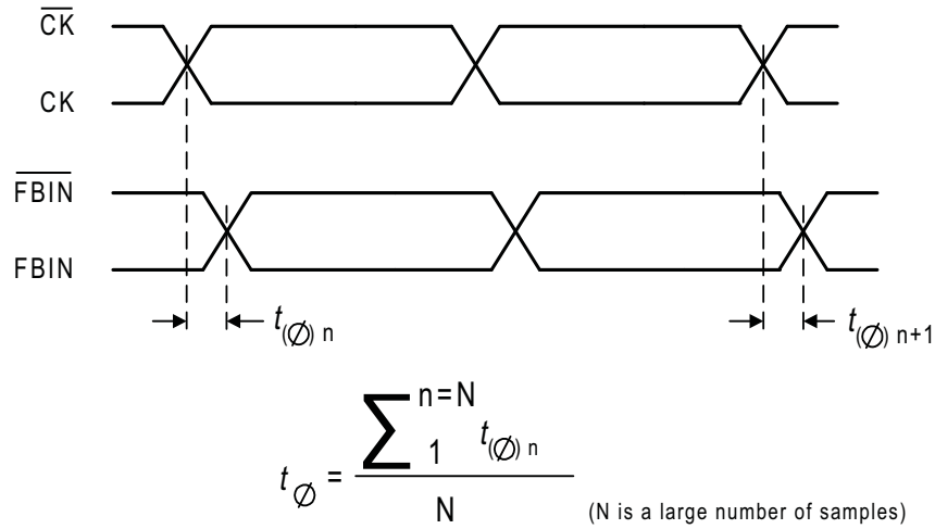
Figure 4. Static Phase Offset
