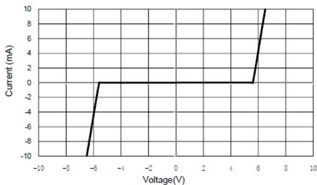
Fig 5 Voltage Sweeping
