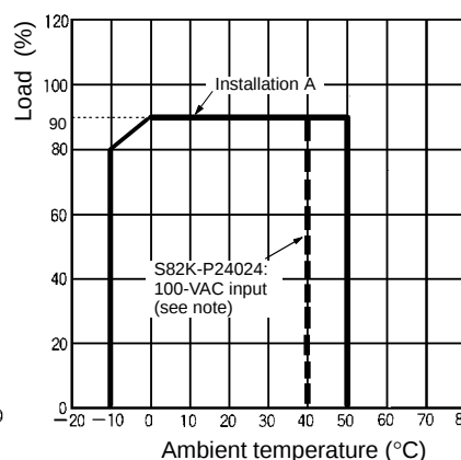
240-W Model Parallel-Unit Operation
