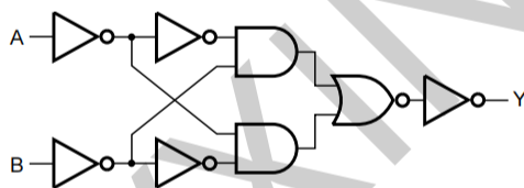
Figure 2. Logic diagram (one gate)
