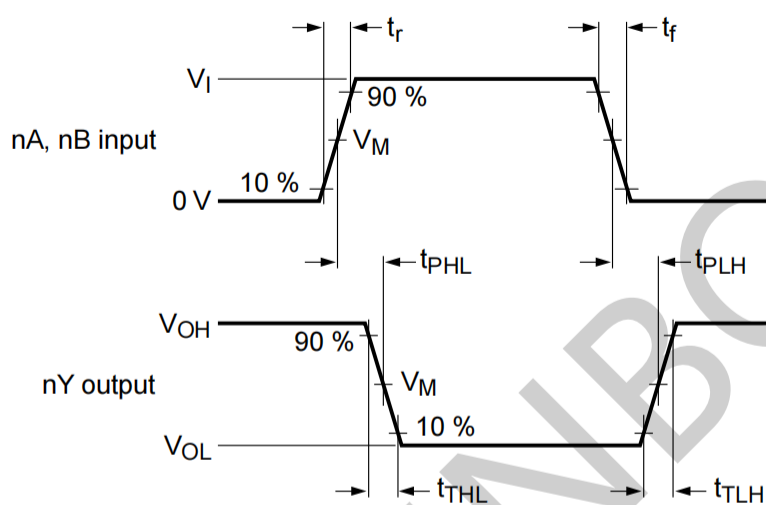
Figure 4. Input to output propagation delays and output transition times
