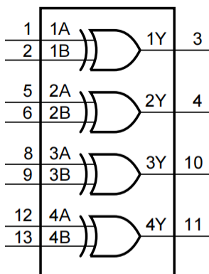
Figure 1. Functional diagram
