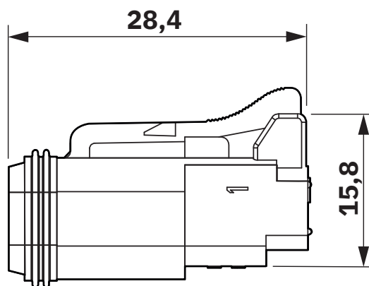
Dimensional drawing
