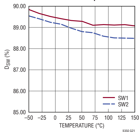
Max On-Time vs Temperature
