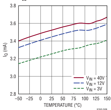
V_{IN} Active Current
