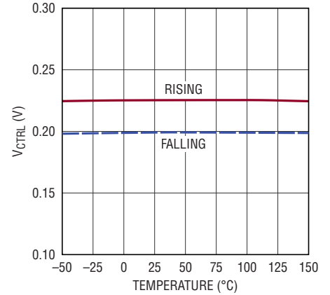
CTRL Off Threshold
