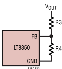
Figure 13. Feedback Resistor Connection
