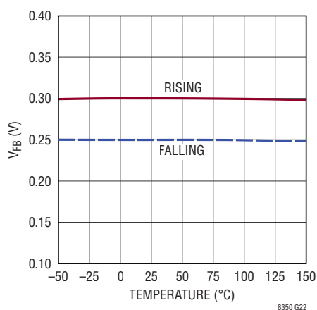
FB Short-Circuit Threshold
