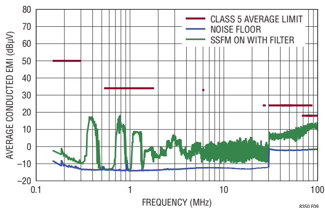
Figure 9. Conducted Average EMI (CISPR25)
