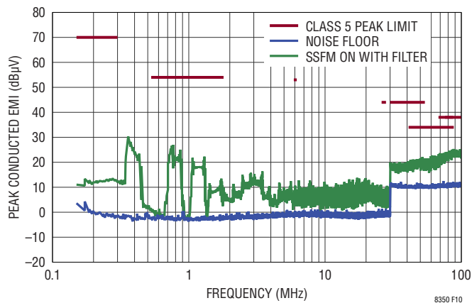
Figure 10. Conducted Peak EMI (CISPR25)
