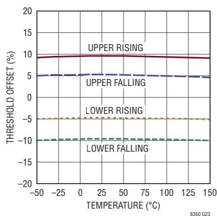
PGOOD Thresholds
