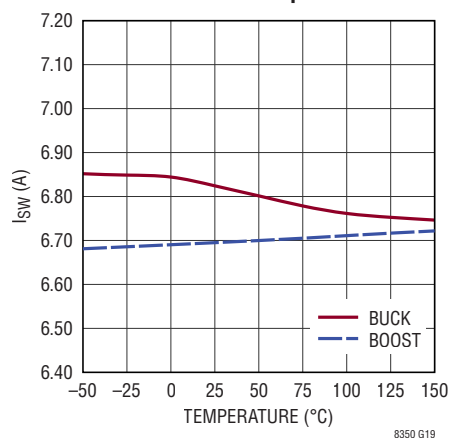
Peak Current vs Temperature
