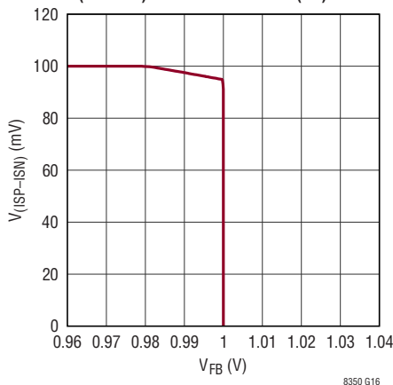
V_{(ISP-ISN)} Regulation vs V_{FB}
