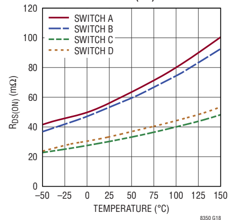
Power Switch R_{DS(ON)}
