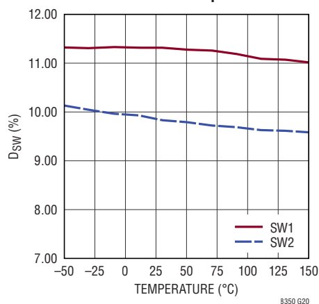
Min On-Time vs Temperature
