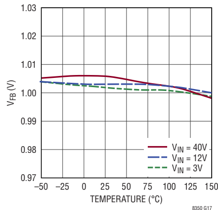
FB Regulation vs Temperature
