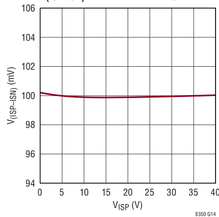
V_{(ISP-ISN)} Regulation vs V_{ISP}
