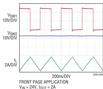
Switching Waveforms (Buck Region)
