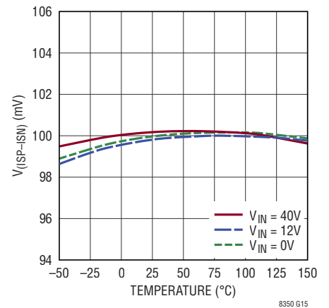
V_{(ISP-ISN)} Regulation vs Temperature
