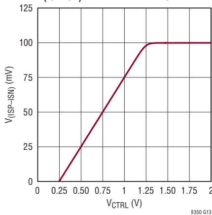
V_{(ISP-ISN)} Regulation vs V_{CTRL}
