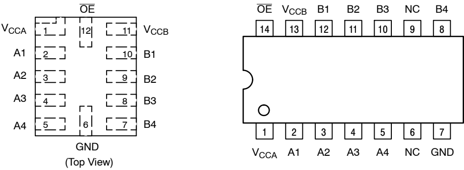
Figure 1. Pin Assignments
