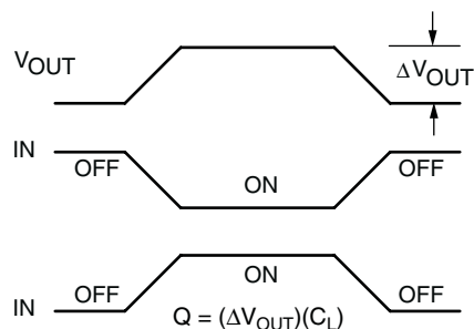
Figure 2. Charge Injection
