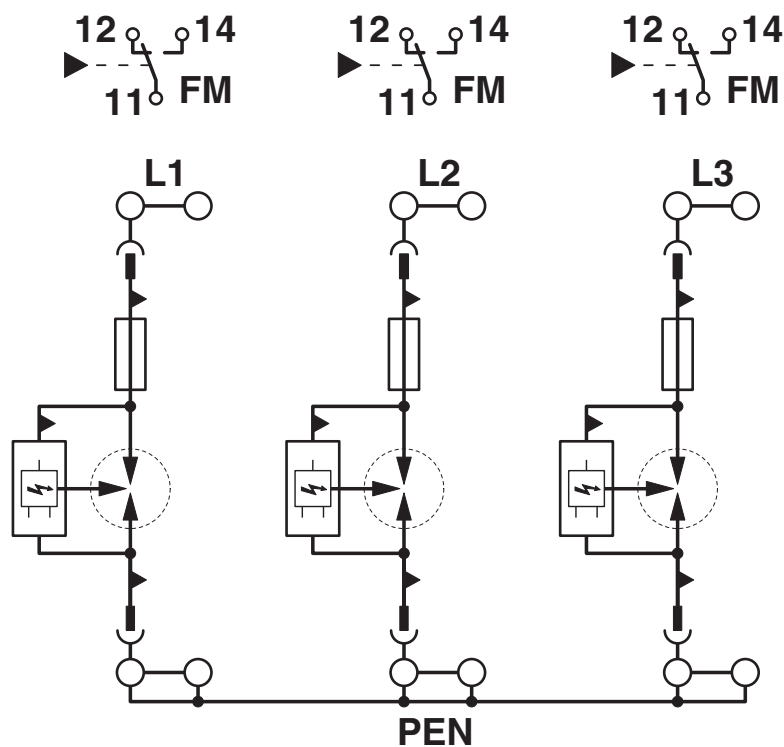
Circuit diagram
