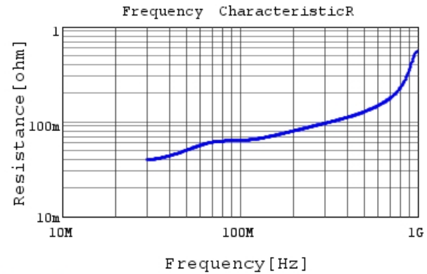
RCE5C2J331J1K1H03B R DCOV, 25degC
