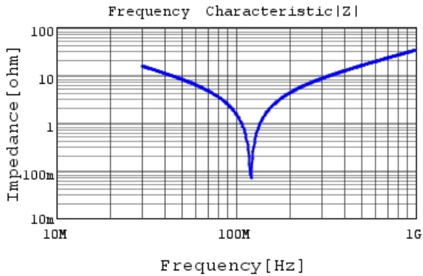
RCE5C2J331J1K1H03B |Z| DCOV, 25degC
