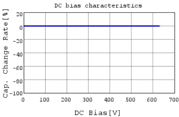
RCE5C2J331J1K1H03B C-DC bias capchange, 25.0
