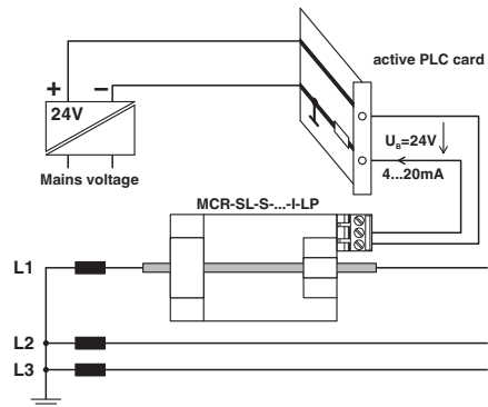
Application drawing
