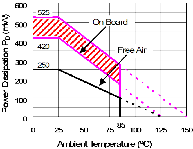
Power Dissipation
