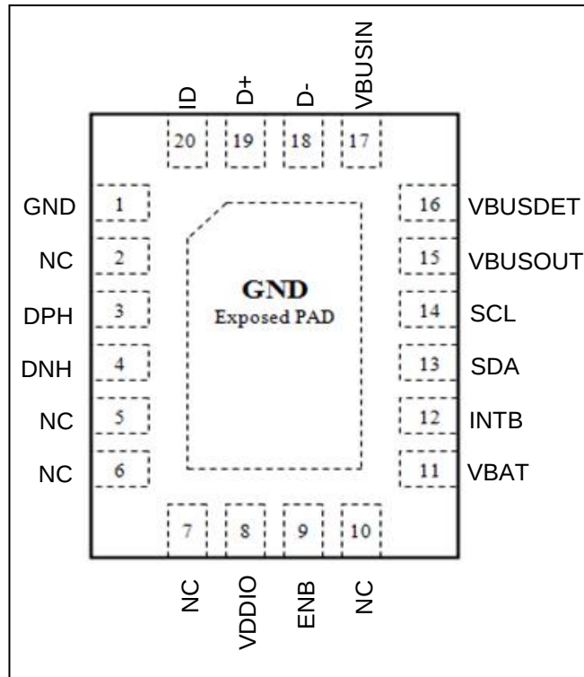
Figure 2b UOFN 20L (3 X 4 X 0.5 mm)
