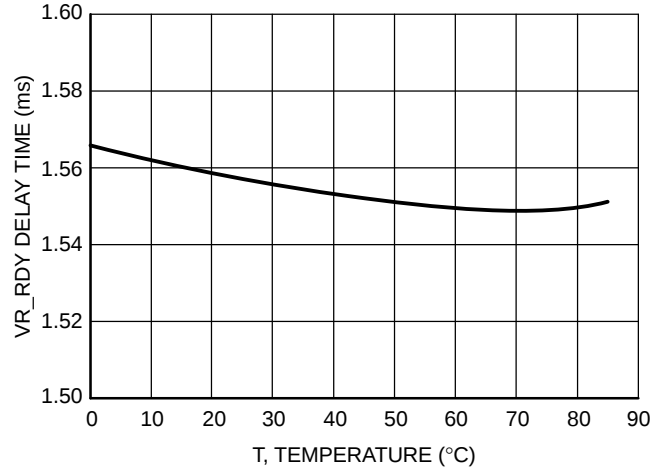
Figure 6. VR Ready Delay Time vs. Temperature
