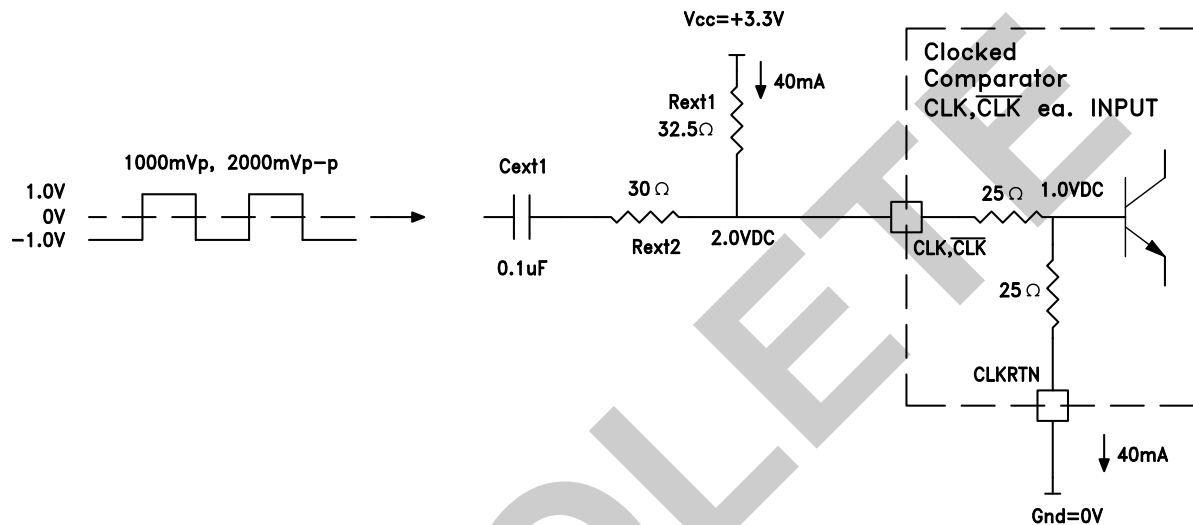
Figure A1: Resistor Network
