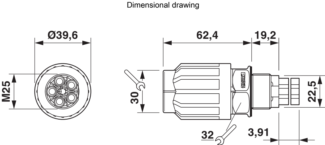
Dimensional drawing of QPD W 4PE6,0 M25
