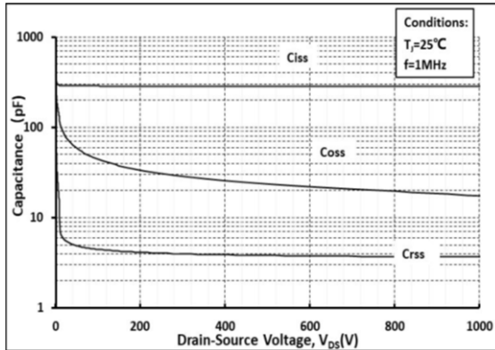
Fig 15: Capacitance Characteristic
