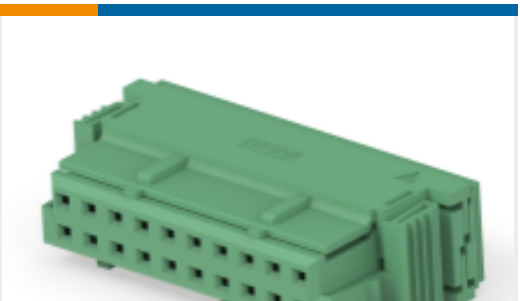
TE Part #374337-E DRBUG B 2,54 20 * CSI 164 E012 ADV J 2
