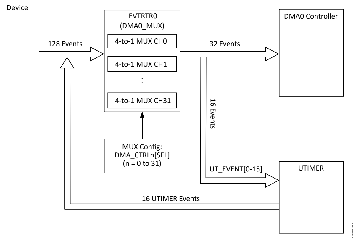
Figure 3-9 EVTRTR Overview
