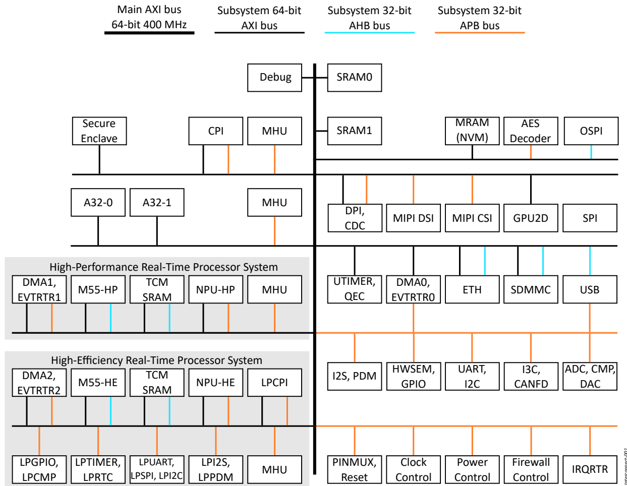
Figure 3-1 Interconnect Overview
