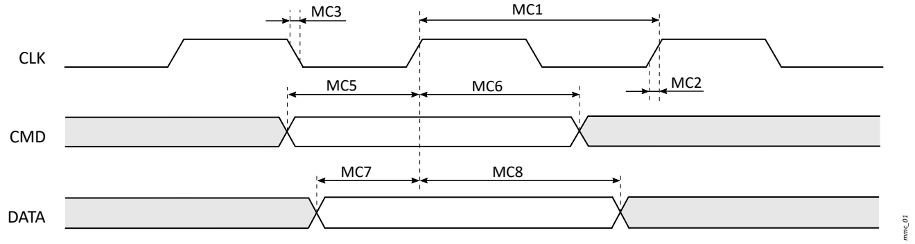
Figure 5-17 SDRAM Timing Diagram (SDR12/SDR25/SDR50)
