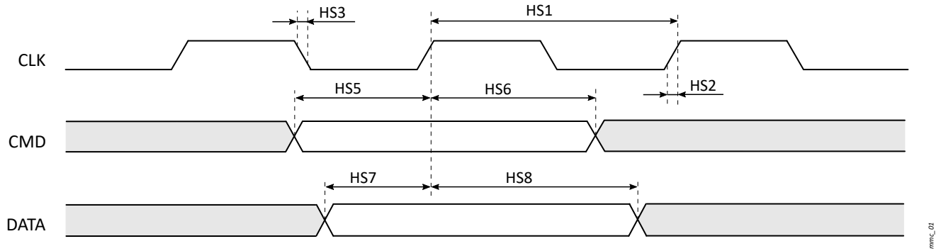
Figure 5-16 SDMMC Timing Diagram (HS mode)
