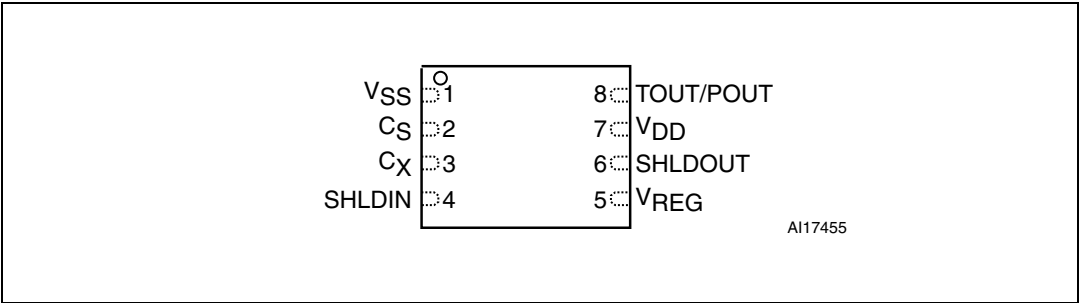
Figure 3. UFDFPN8 pinout
