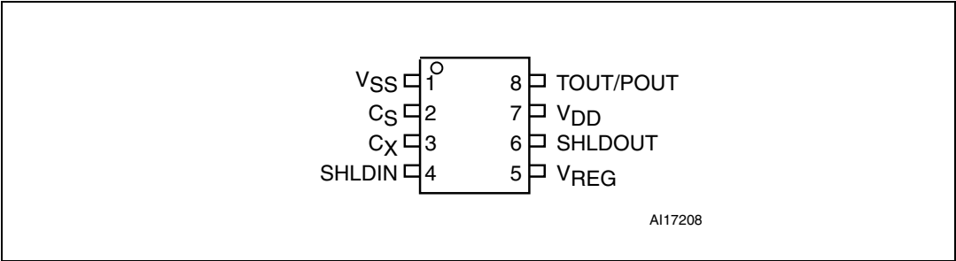
Figure 2. S08 pinout
