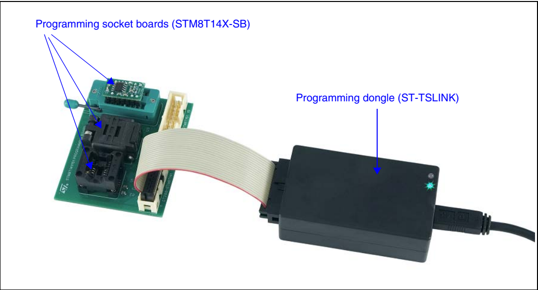
Figure 29. STM8T141-EVAL programming tool
